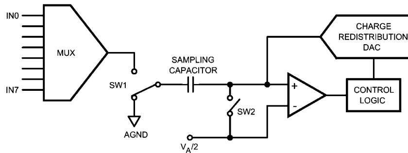
FIGURE 5. ADC128S052 in Hold Mode
